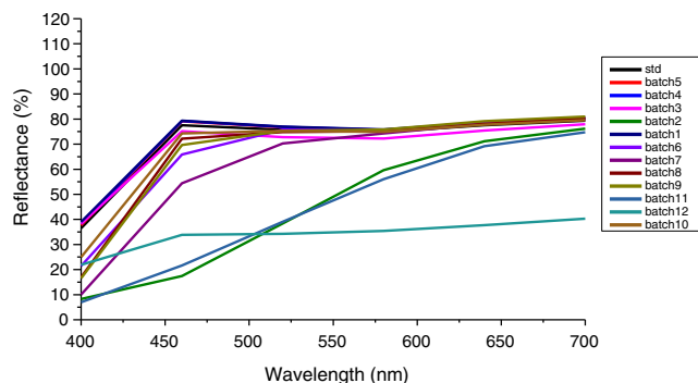
Fig. 1 Combined Reflectance Spectra of Synthesized OBAs
